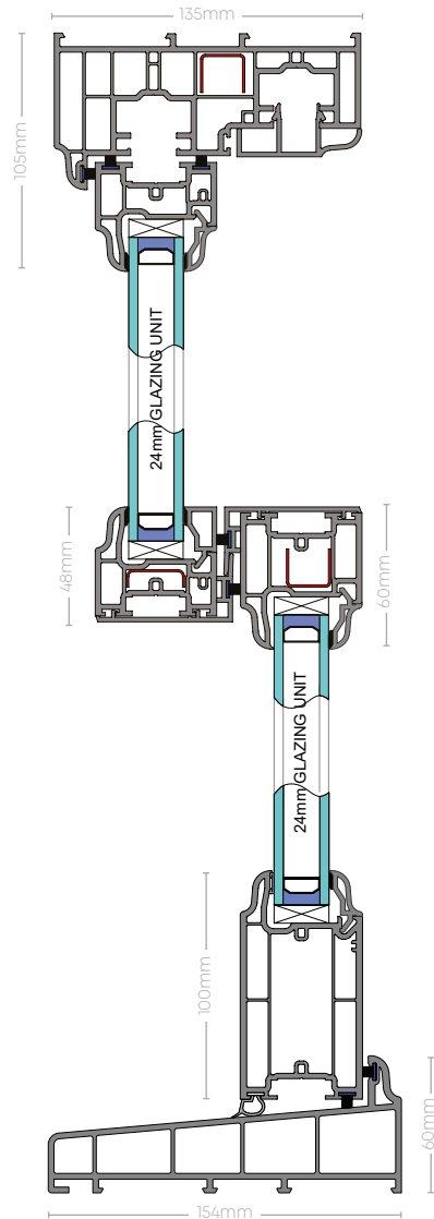
Vertical section through sash with DBR and non standard sill option
